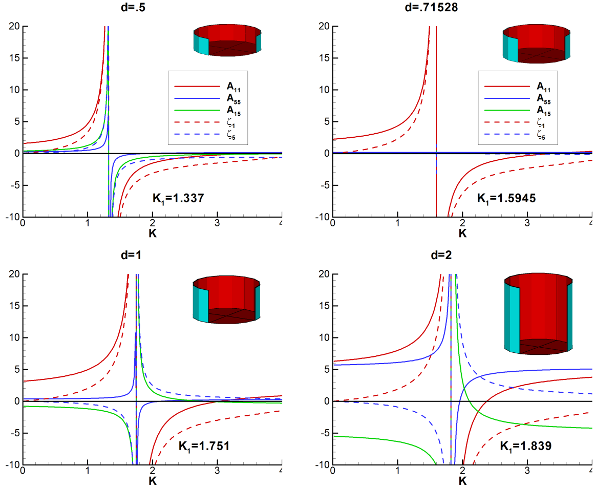
Figure 1: Added-mass coefficients ( A_{ij} ) and sloshing amplitudes ( \zeta_i ) for forced oscillatory motion of the tank with no exterior fluid domain. The mode index i = 1 for surge and i = 5 for pitch. The value of the resonant wavenumber K_1 is shown for each tank. In the perspective figures one quadrant of the side is removed to show the interior.
