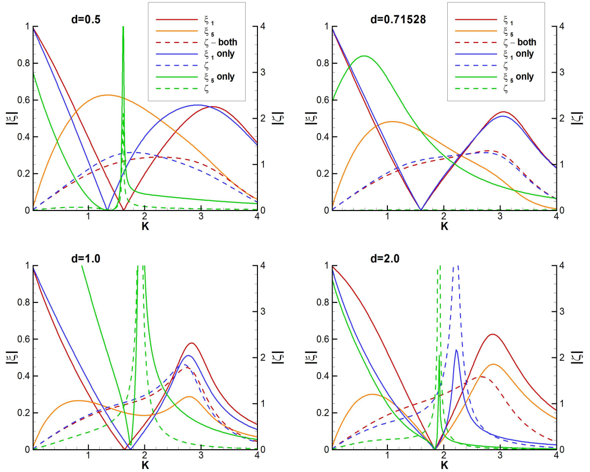
Figure 2: Free motions in waves and sloshing amplitude. The RAOs |\xi_i| are shown by the solid lines and measured by the left axis. The sloshing amplitude |\zeta| is shown by the dashed lines and the right axis.
