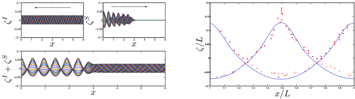
Figure 3: Nonlinear standing waves by reflection from a wall. Left: The two components and their sum. Right: Comparison with experiments by [7] for the steepest stable standing wave.
